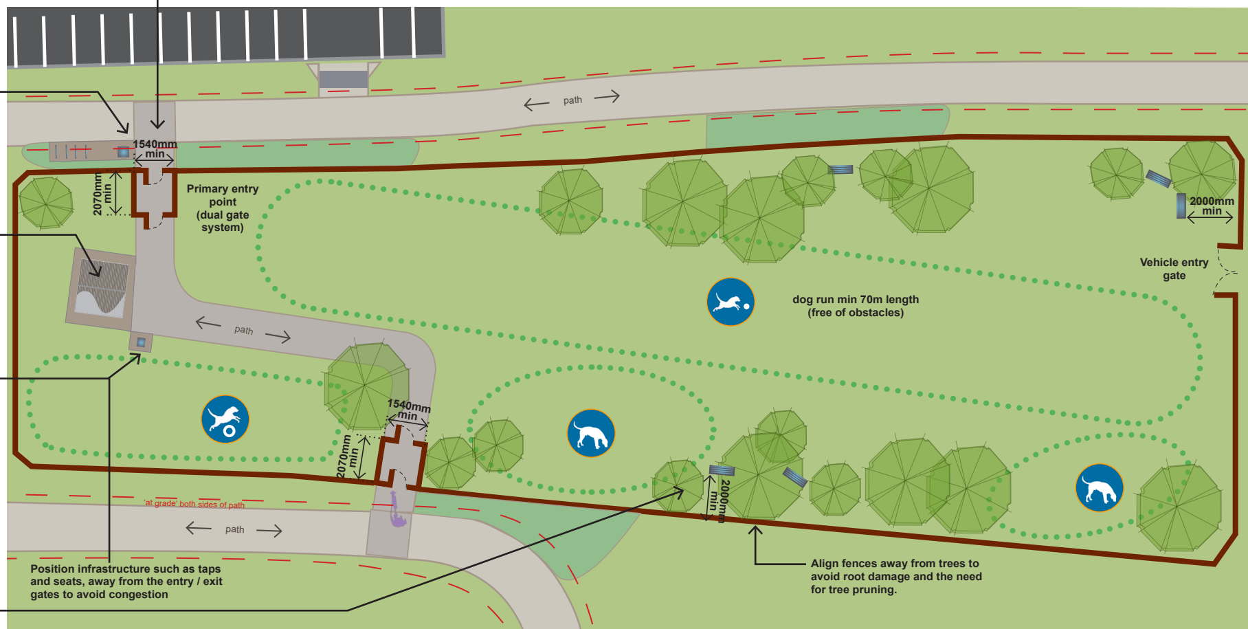
Figure 14: Example plan – Fenced (off leash) DEA (not to scale – for guidance only – site specific design required)
